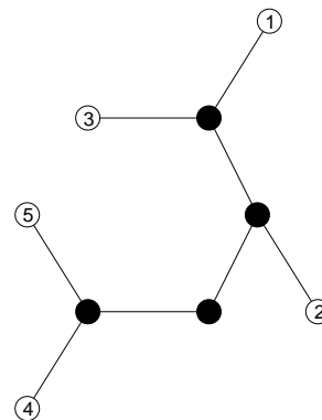
Figure 1: A connected backbone does not necessarily preserve capacity. In this connected topology, black nodes are coordinators. Packets between nodes 3 and 4 may contend for bandwidth with packets between nodes 1 and 2. On the other hand, if node 5 were a coordinator, no contention would occur.
