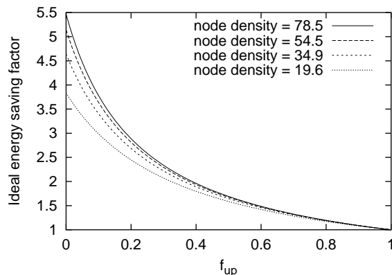
Figure 10: Energy savings as a function of f_{up} , computed using Equation 5, substituting C_{ideal} and 0.157 as values for C and \alpha . This figure shows that as f_{up} increases, the amount of energy saving decreases as well. In our experiments, f_{up} was between 0.185 and 0.263.
