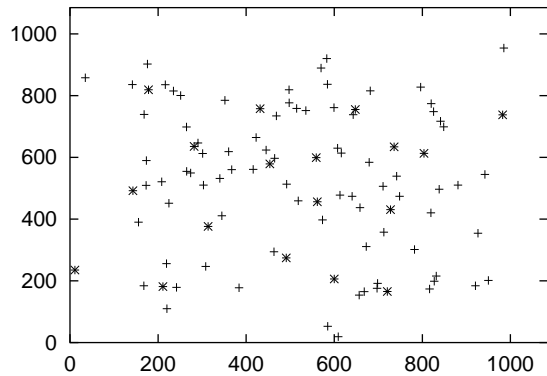
Figure 3: A scenario with 100 nodes, 18 coordinators, and a radio range of 250 meters. The nodes marked “*” are coordinators; the nodes marked “+” are non-coordinator nodes.
